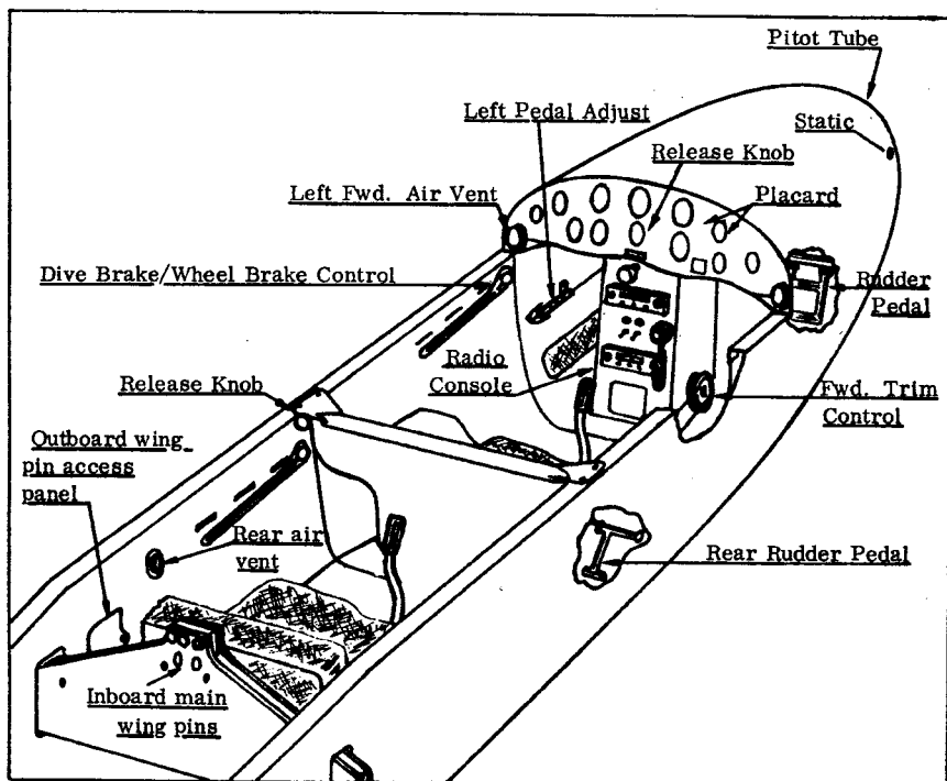
SGS 2-32 Cockpit (Instruments & Controls)
